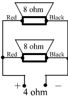
Parallel schakeling van 2 speakers
